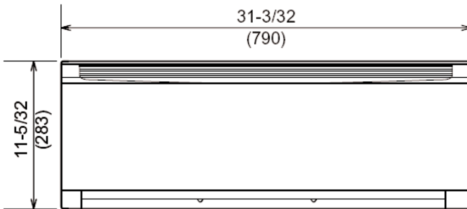
Front view
